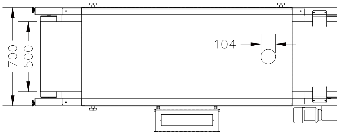
ELECTRIC TUNNEL DRYER ECONO-2060 MAIN VIEW
