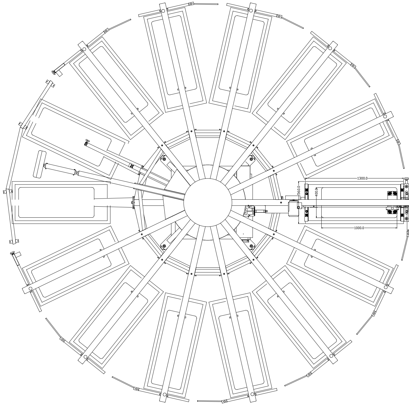
PRISM I 14s 12c 40 x 90 cm print area configuration
